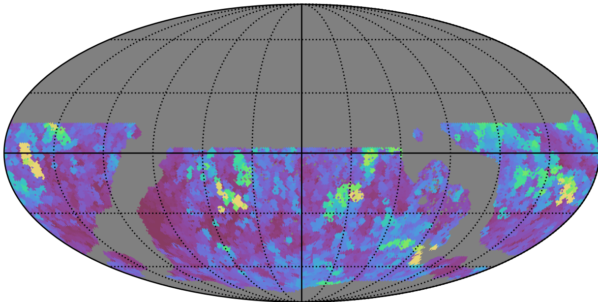
ddf_loaded_fl4_v3.4_10yrs WFD z band: Max seeingEff
