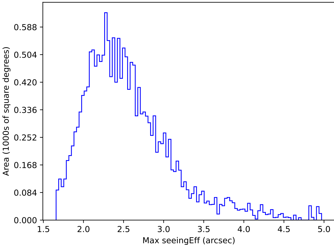
ddf_loaded_fl4_v3.4_10yrs WFD z band: Max seeingEff
