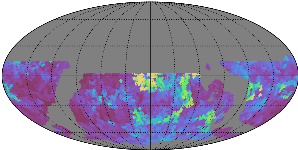
ddf_loaded_fl4_v3.4_10yrs WFD y band: Max seeingEff
