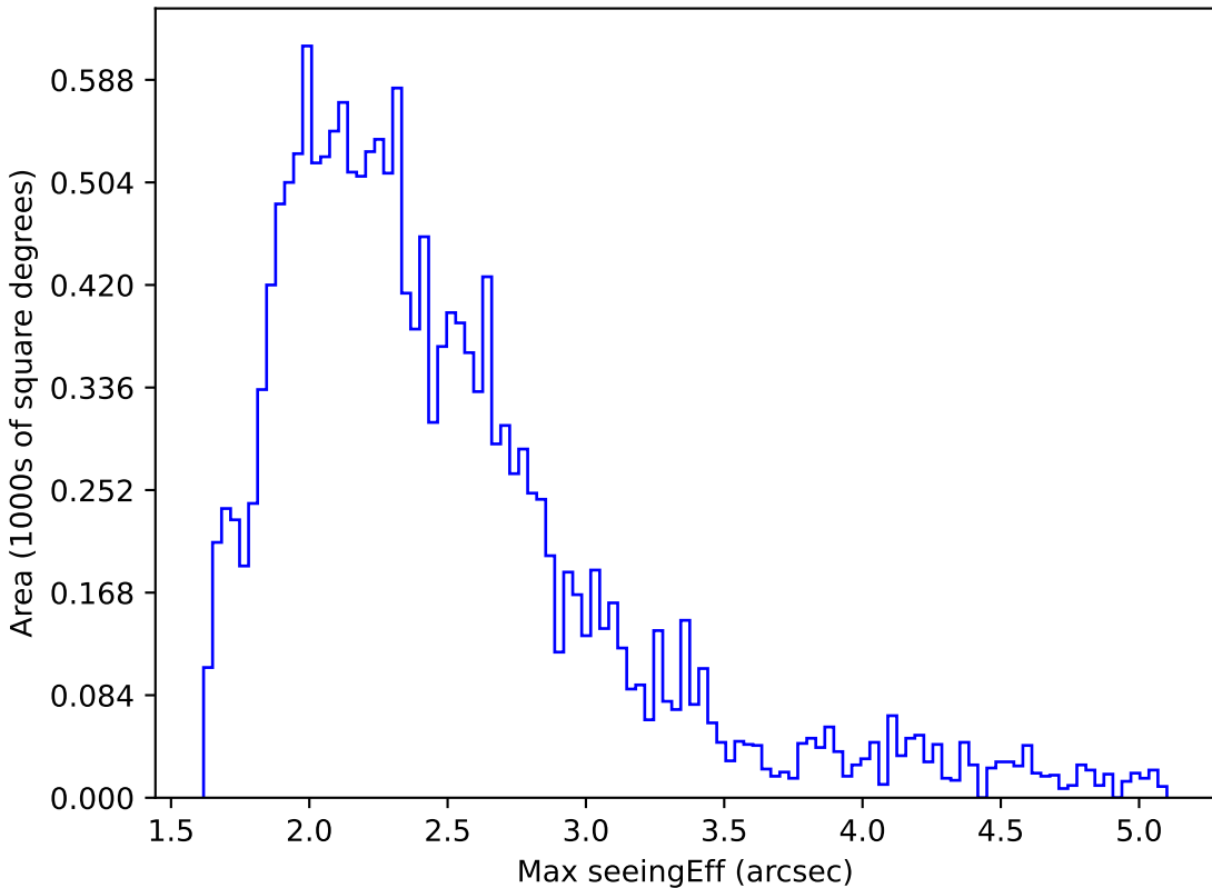
ddf_loaded_fl4_v3.4_10yrs WFD y band: Max seeingEff
