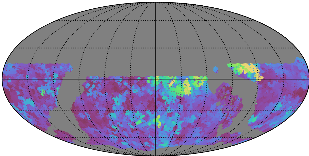
ddf_loaded_fl4_v3.4_10yrs WFD u band: Max seeingEff
