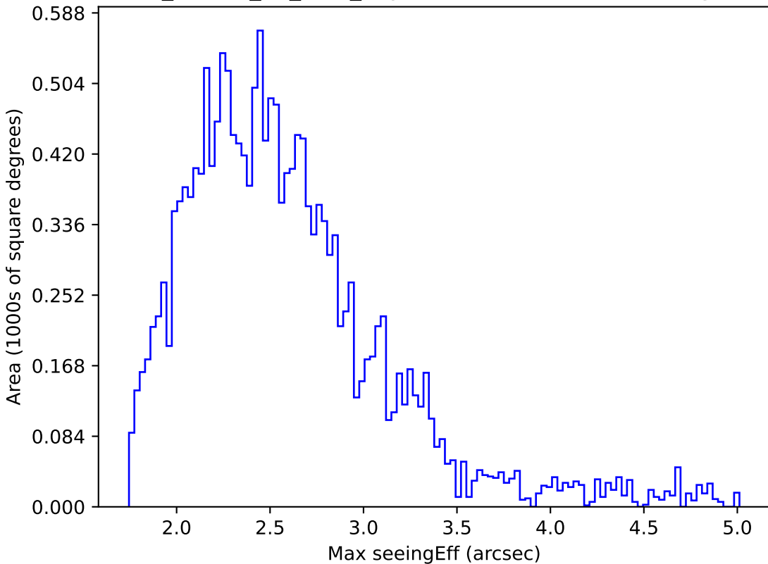
ddf_loaded_fl4_v3.4_10yrs WFD u band: Max seeingEff
