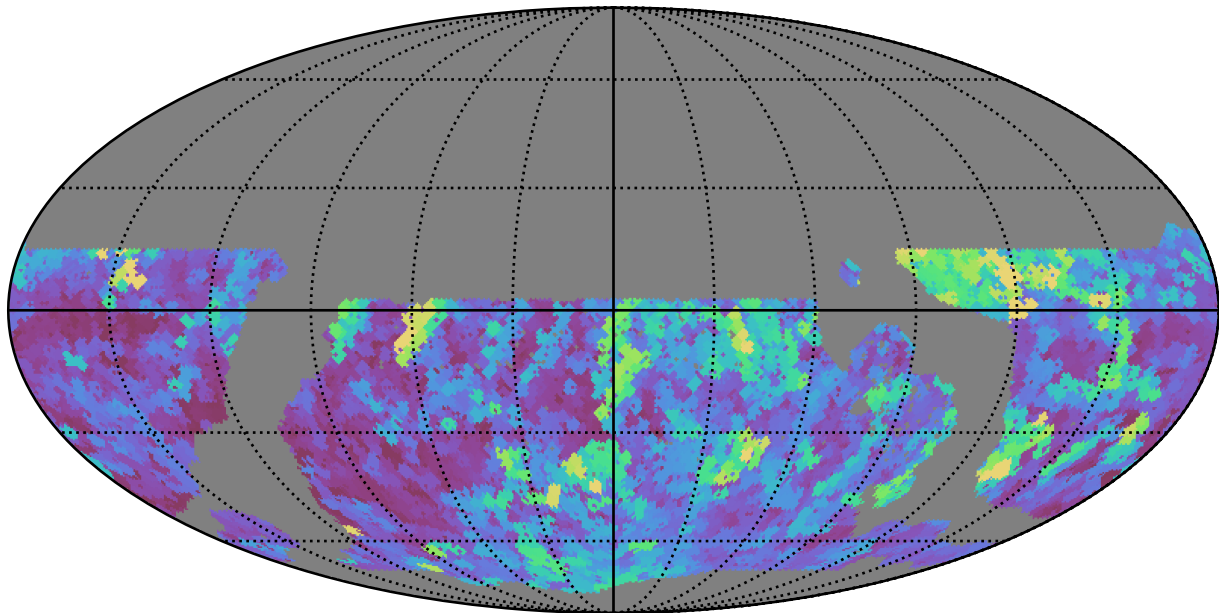
ddf_loaded_fl4_v3.4_10yrs WFD r band: Max seeingEff
