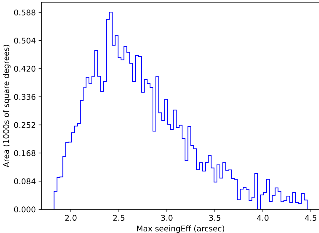
ddf_loaded_fl4_v3.4_10yrs WFD r band: Max seeingEff
