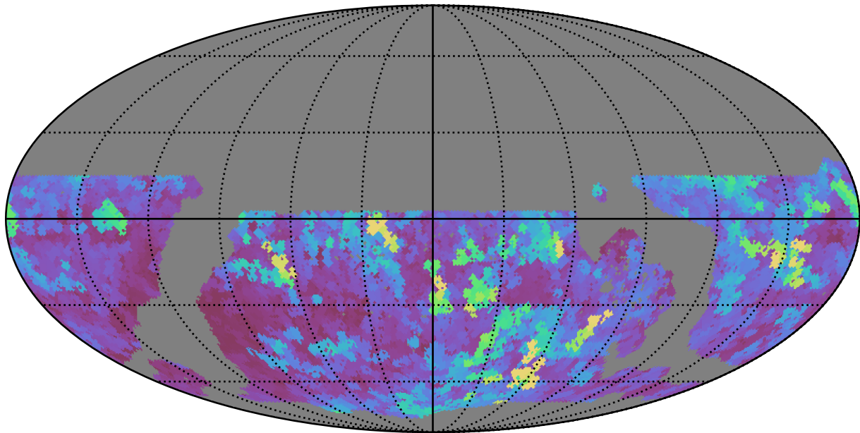
ddf_loaded_fl4_v3.4_10yrs WFD i band: Max seeingEff
