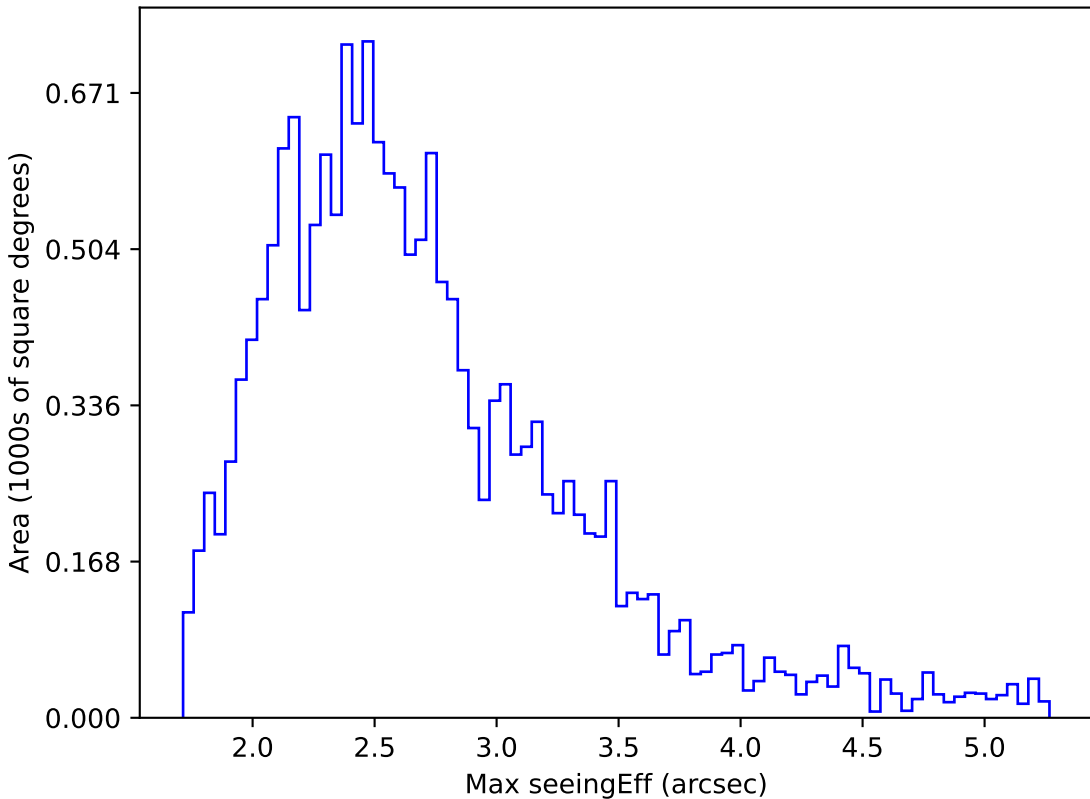
ddf_loaded_fl4_v3.4_10yrs WFD i band: Max seeingEff
