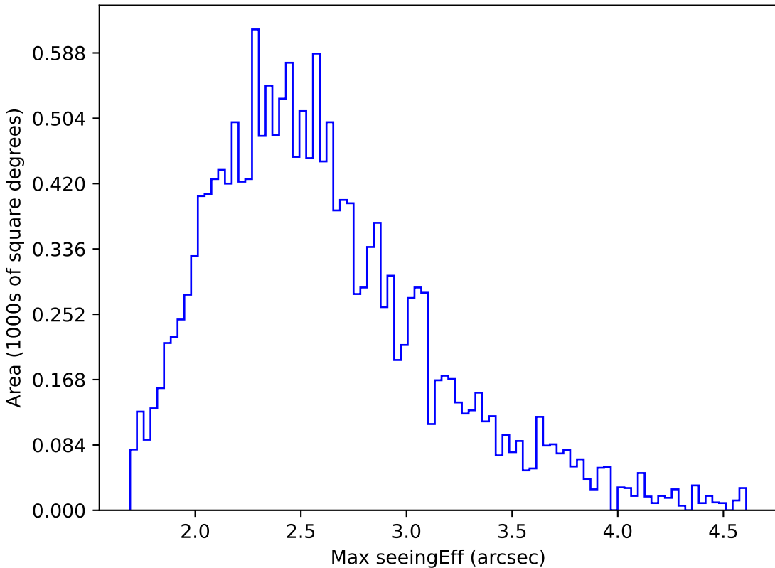
ddf_loaded_fl4_v3.4_10yrs WFD g band: Max seeingEff
