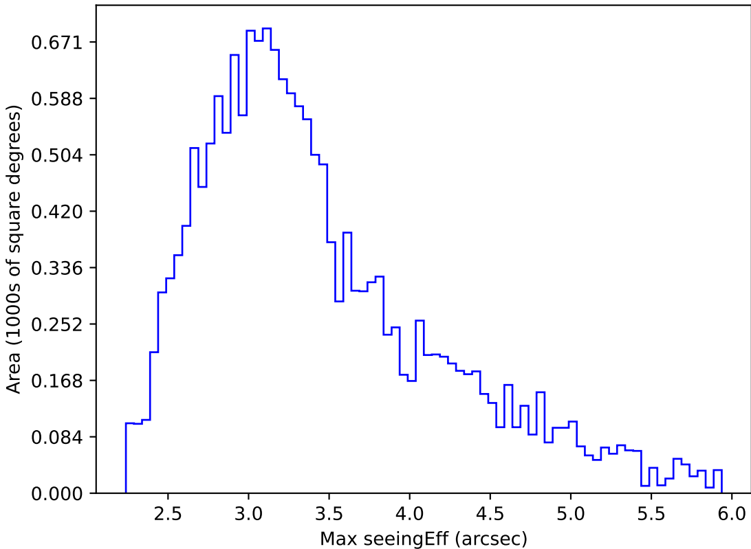
ddf_loaded_fl4_v3.4_10yrs WFD all bands: Max seeingEff
