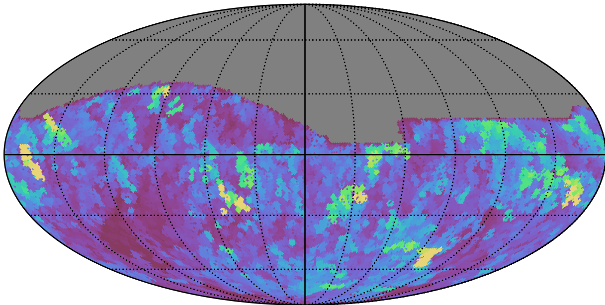
ddf_loaded_fl4_v3.4_10yrs All sky z band: Max seeingEff
