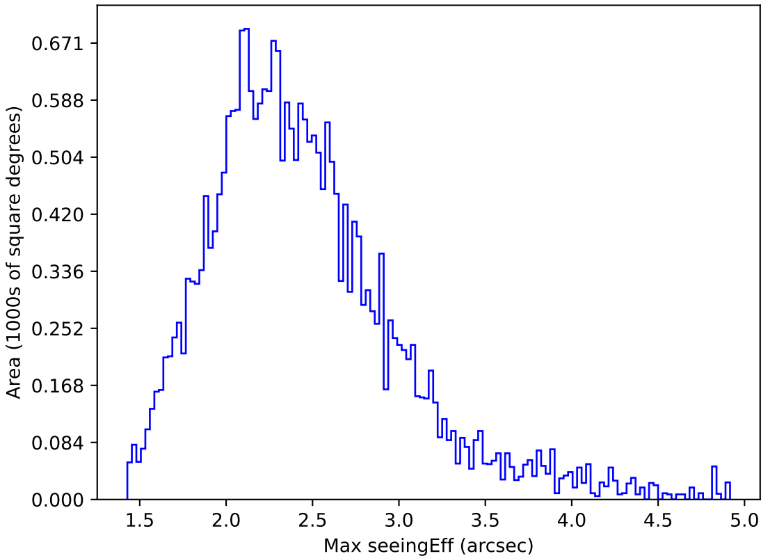
ddf_loaded_fl4_v3.4_10yrs All sky z band: Max seeingEff
