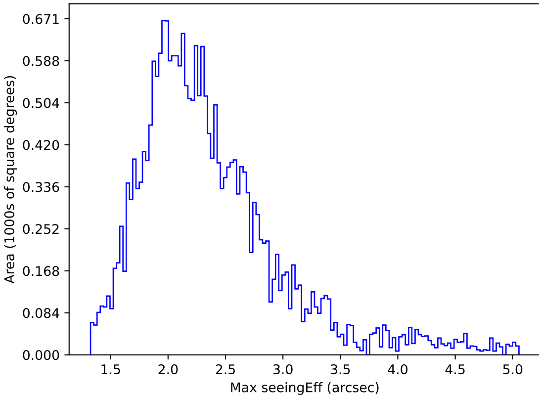
ddf_loaded_fl4_v3.4_10yrs All sky y band: Max seeingEff
