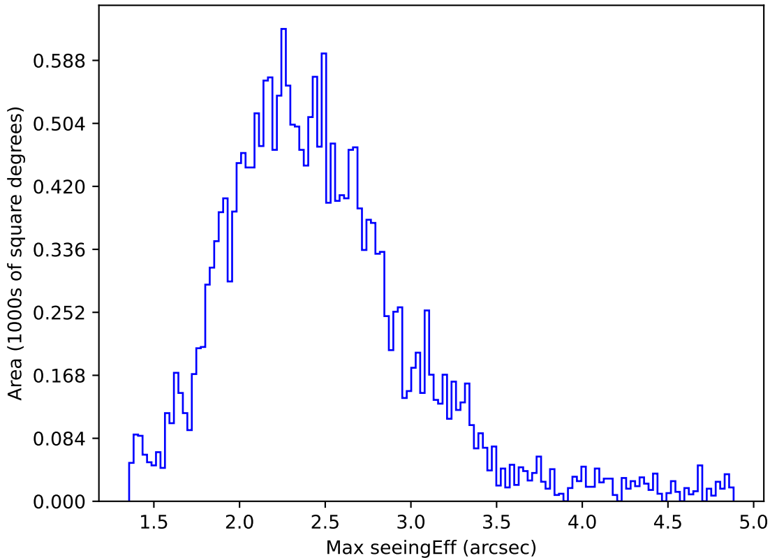
ddf_loaded_fl4_v3.4_10yrs All sky u band: Max seeingEff
