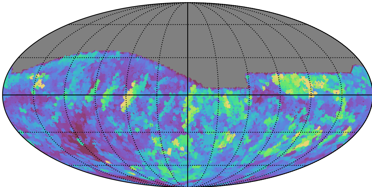
ddf_loaded_fl4_v3.4_10yrs All sky r band: Max seeingEff
