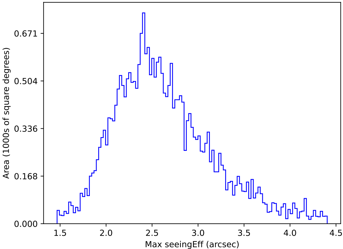
ddf_loaded_fl4_v3.4_10yrs All sky r band: Max seeingEff
