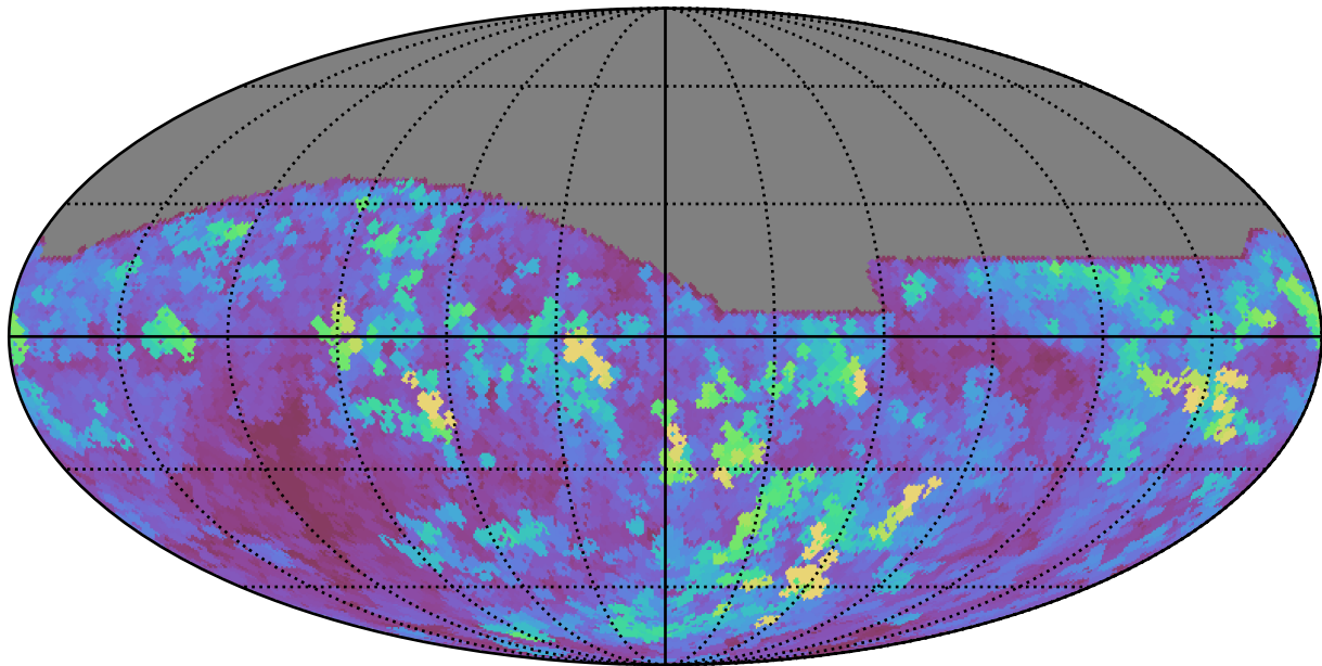
ddf_loaded_fl4_v3.4_10yrs All sky i band: Max seeingEff
