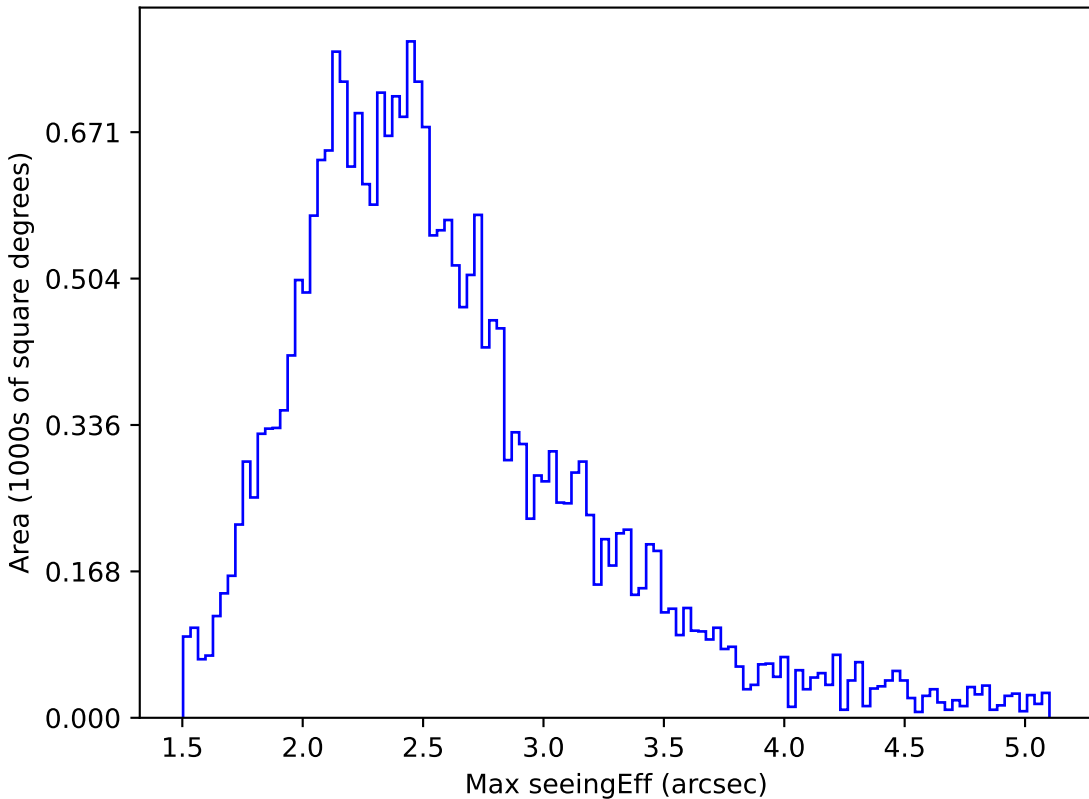
ddf_loaded_fl4_v3.4_10yrs All sky i band: Max seeingEff
