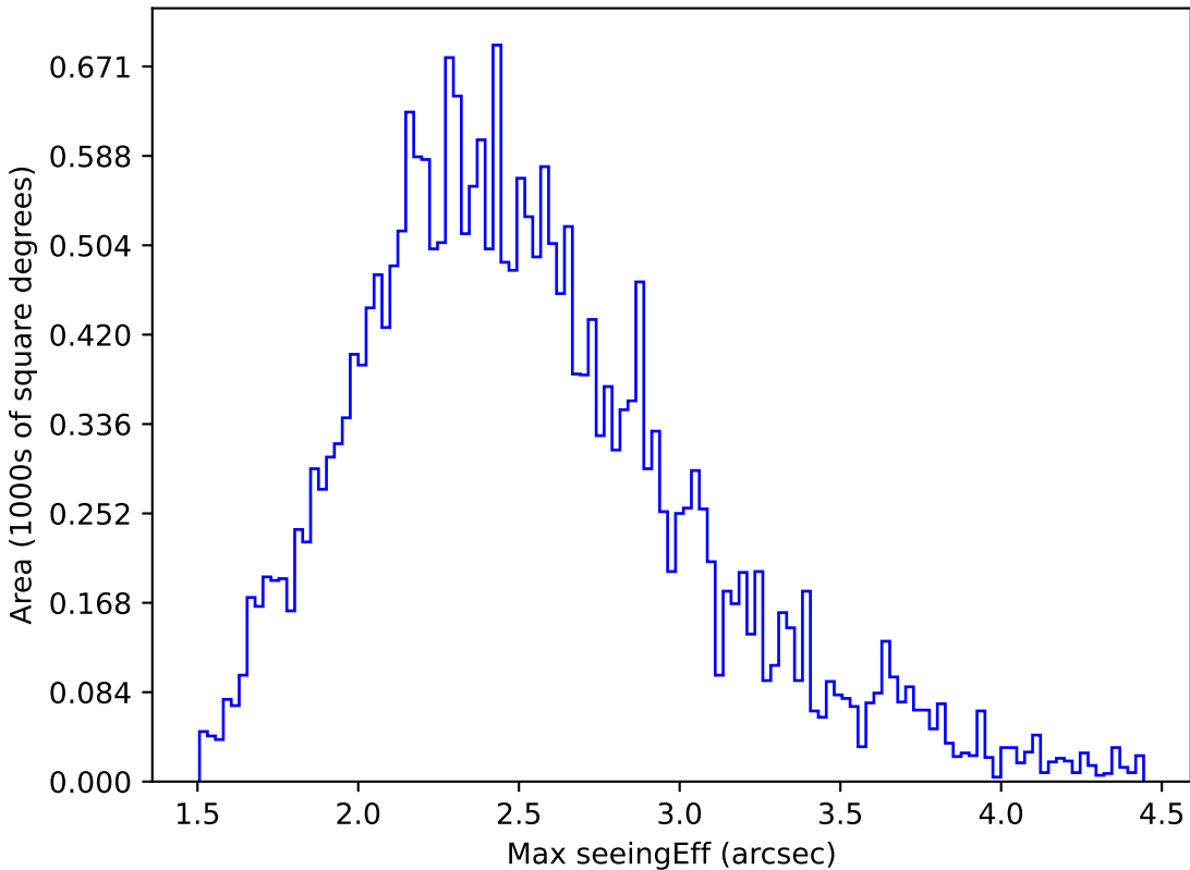
ddf_loaded_fl4_v3.4_10yrs All sky g band: Max seeingEff
