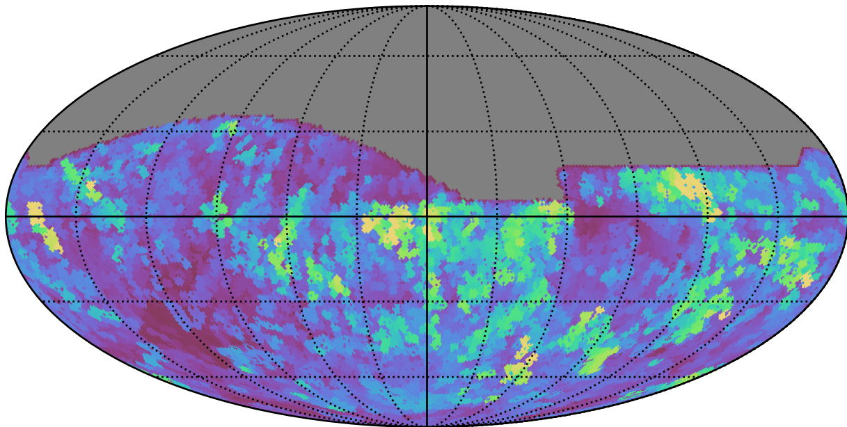
ddf_loaded_fl4_v3.4_10yrs All sky all bands: Max seeingEff
