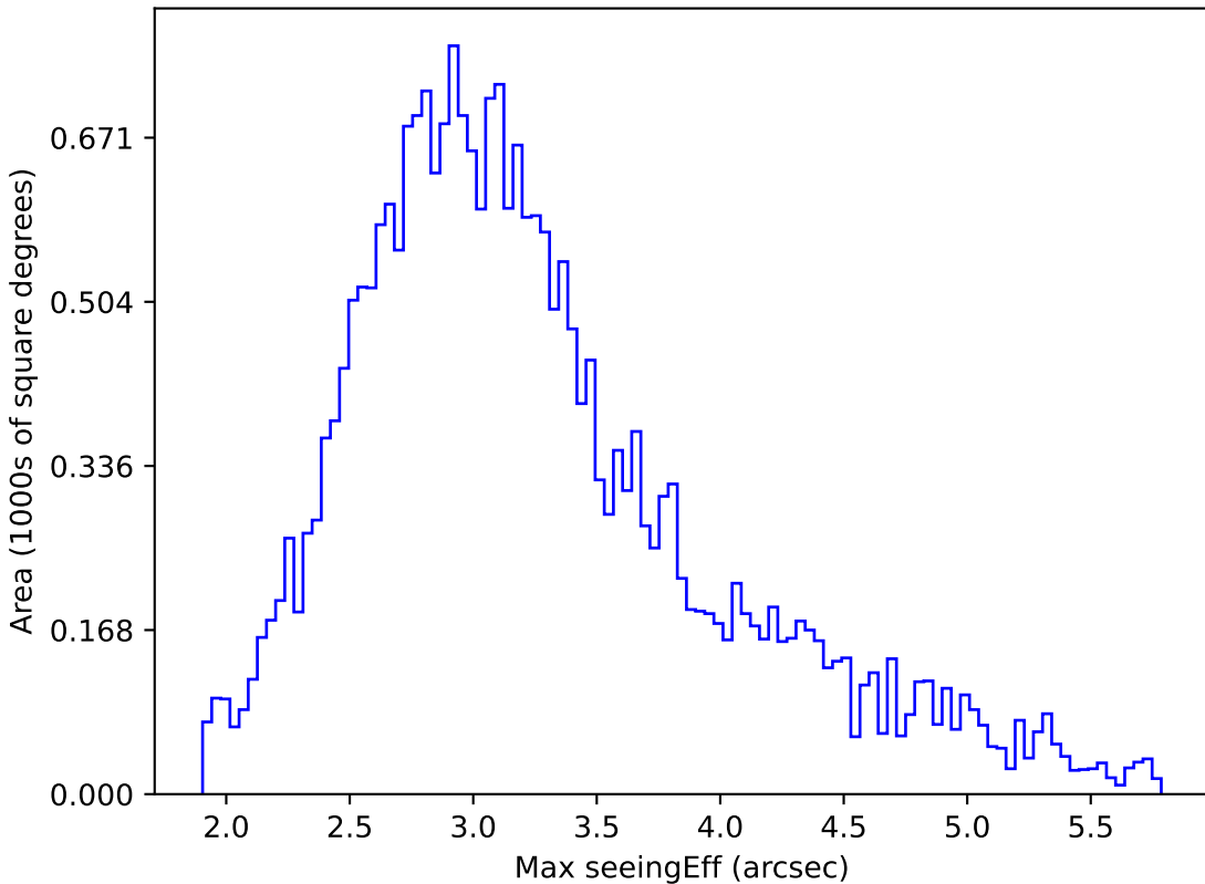
ddf_loaded_fl4_v3.4_10yrs All sky all bands: Max seeingEff
