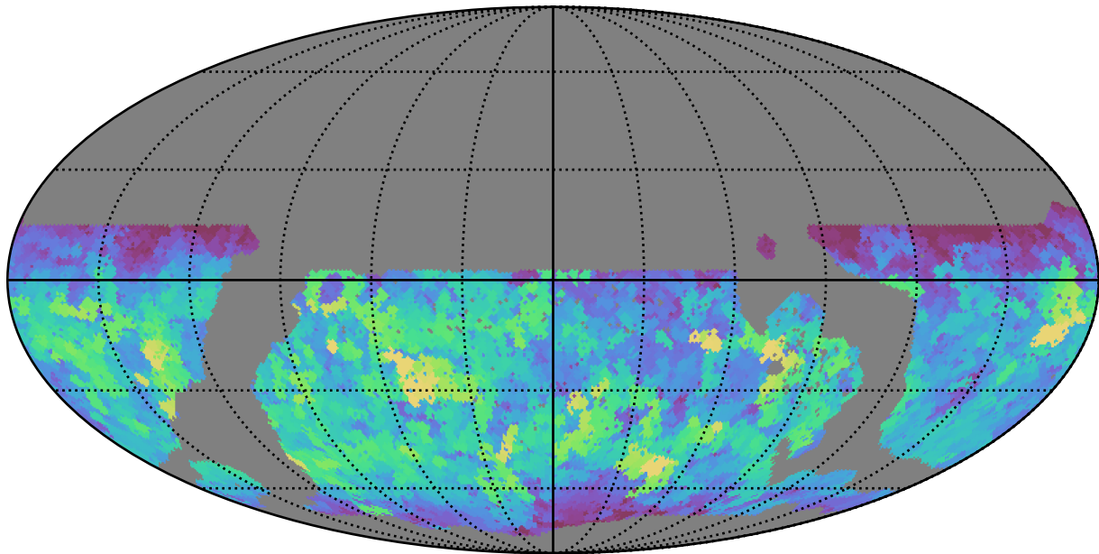
ddf_loaded_fl4_v3.4_10yrs WFD z band: Max saturation_mag
