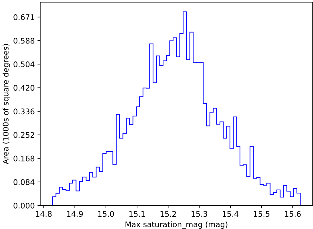
ddf_loaded_fl4_v3.4_10yrs WFD z band: Max saturation_mag
