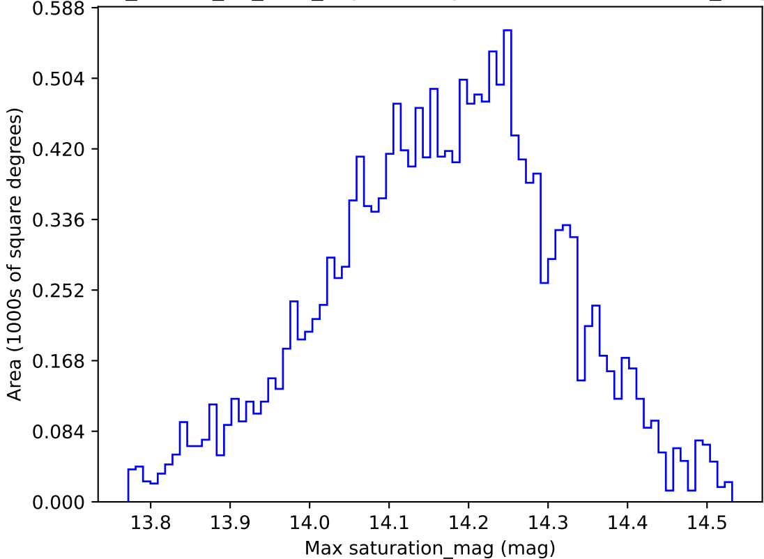
ddf_loaded_fl4_v3.4_10yrs WFD y band: Max saturation_mag
