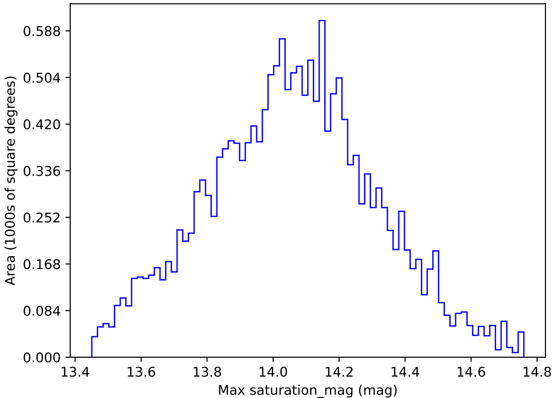
ddf_loaded_fl4_v3.4_10yrs WFD u band: Max saturation_mag
