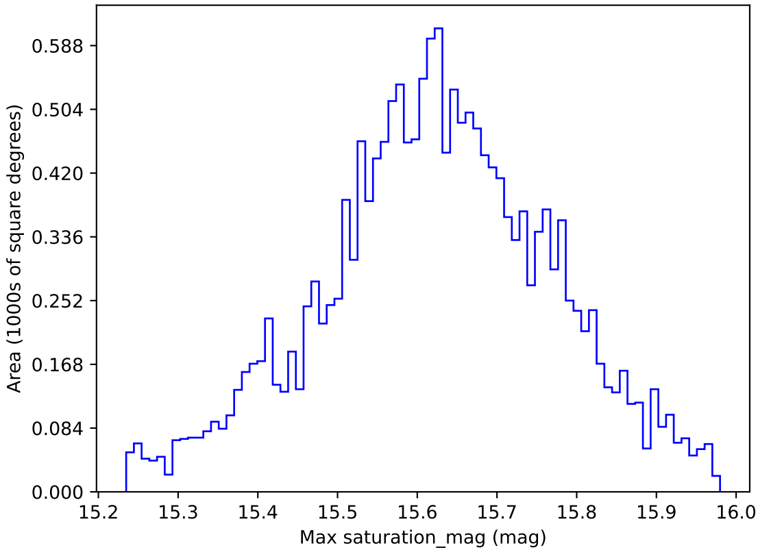
ddf_loaded_fl4_v3.4_10yrs WFD i band: Max saturation_mag
