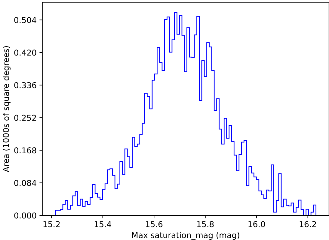
ddf_loaded_fl4_v3.4_10yrs WFD g band: Max saturation_mag
