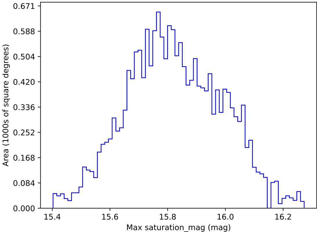
ddf_loaded_fl4_v3.4_10yrs WFD all bands: Max saturation_mag
