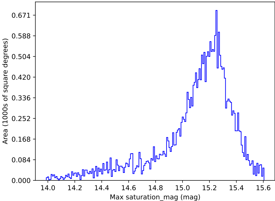
ddf_loaded_fl4_v3.4_10yrs All sky z band: Max saturation_mag
