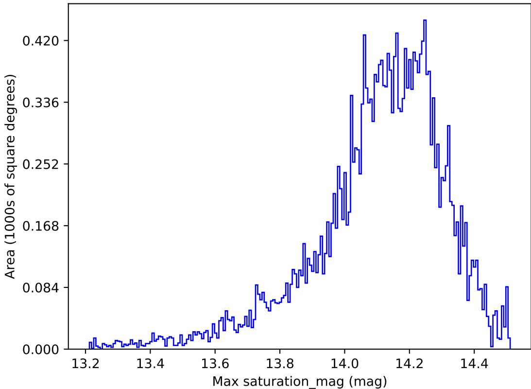
ddf_loaded_fl4_v3.4_10yrs All sky y band: Max saturation_mag
