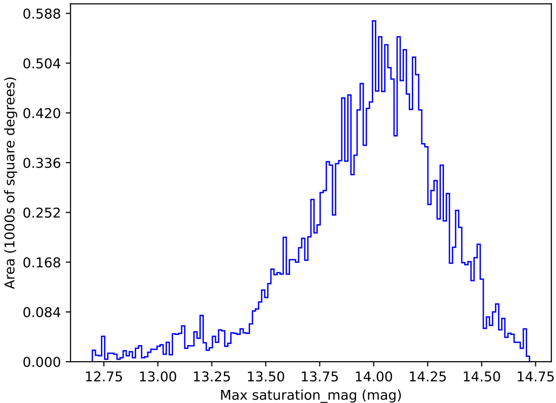
ddf_loaded_fl4_v3.4_10yrs All sky u band: Max saturation_mag
