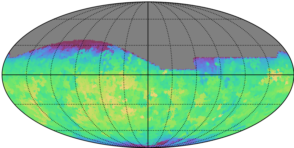
ddf_loaded_fl4_v3.4_10yrs All sky r band: Max saturation_mag
