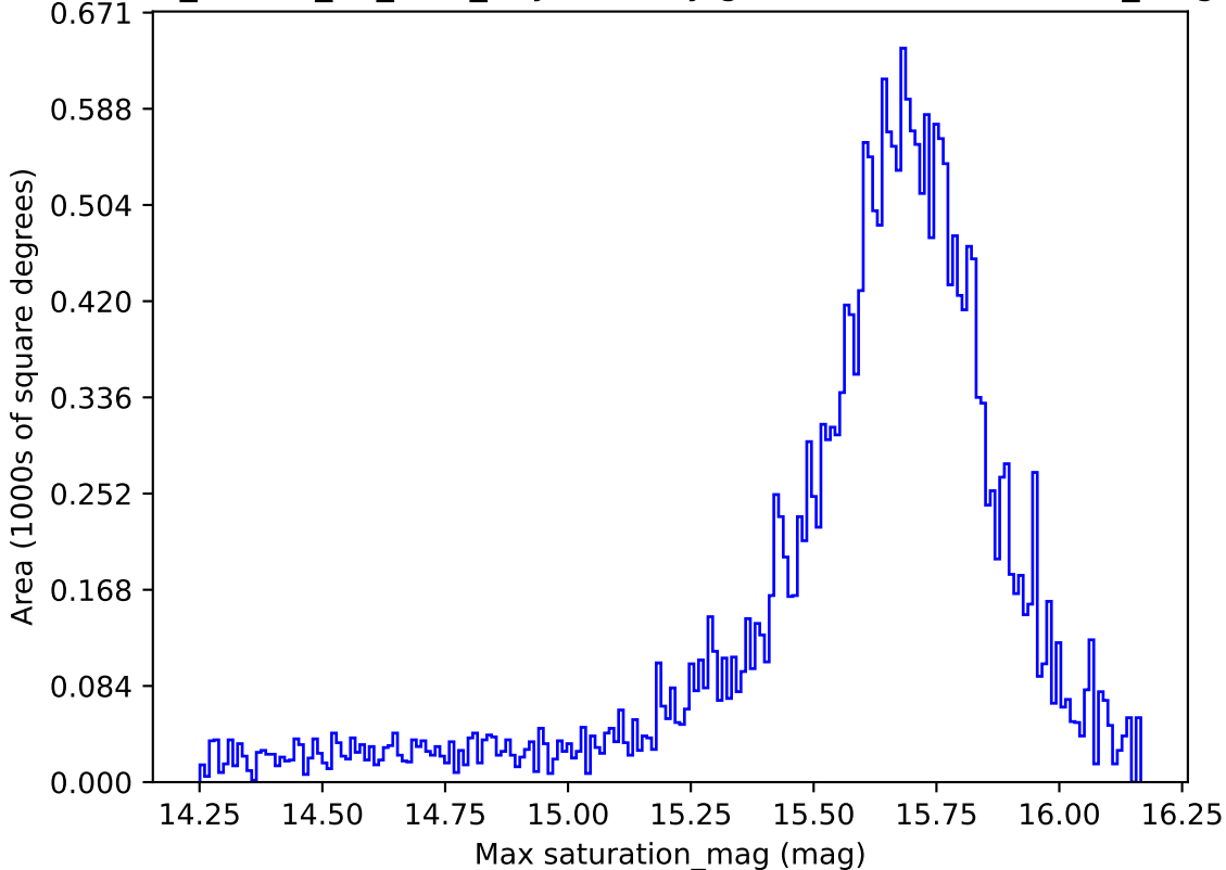
ddf_loaded_fl4_v3.4_10yrs All sky g band: Max saturation_mag
