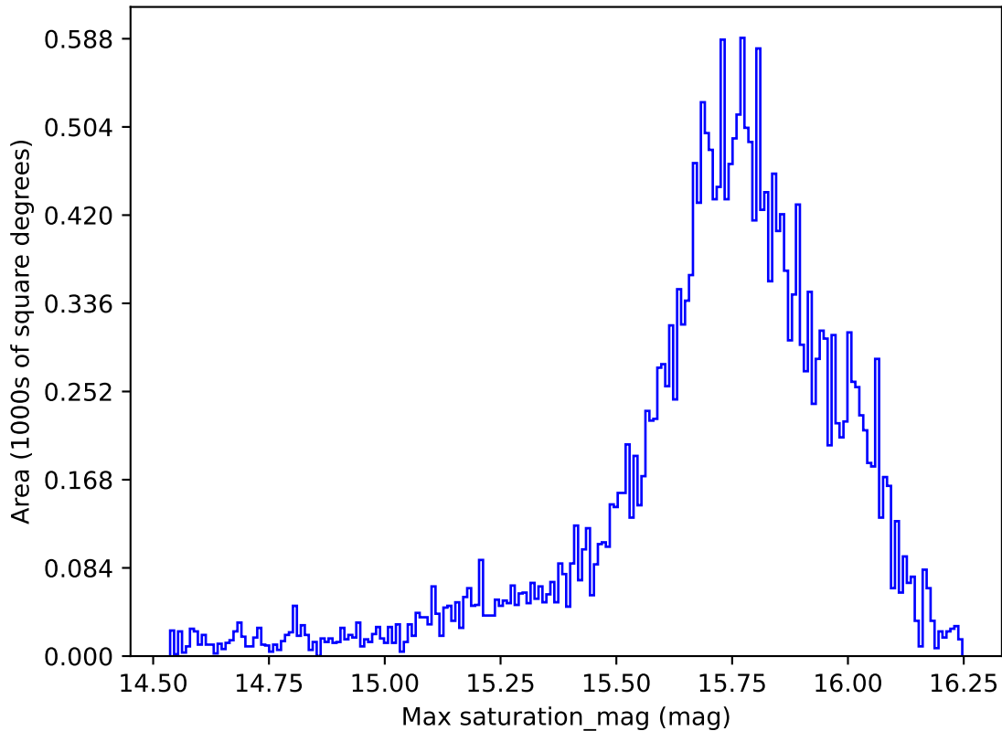
ddf_loaded_fl4_v3.4_10yrs All sky all bands: Max saturation_mag
