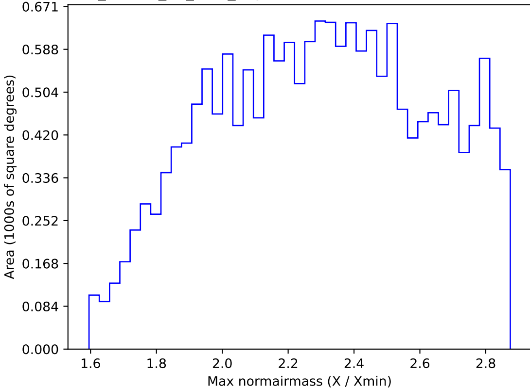
ddf_loaded_fl4_v3.4_10yrs WFD z band: Max normairmass
