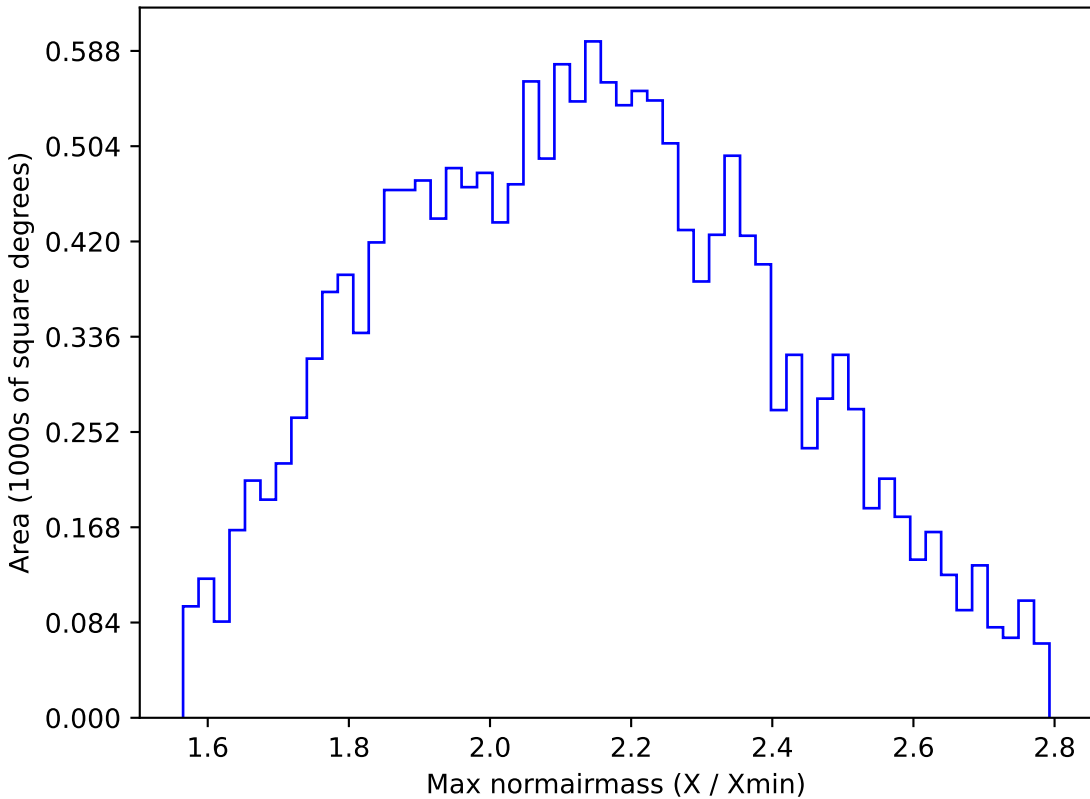
ddf_loaded_fl4_v3.4_10yrs WFD y band: Max normairmass
