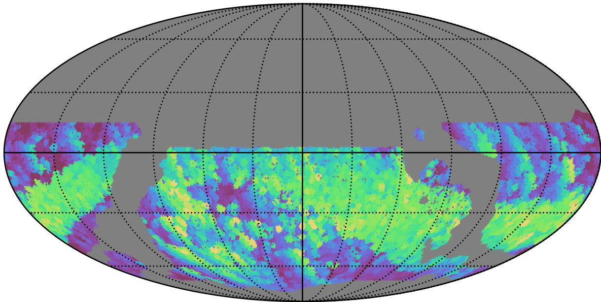
ddf_loaded_fl4_v3.4_10yrs WFD r band: Max normairmass
