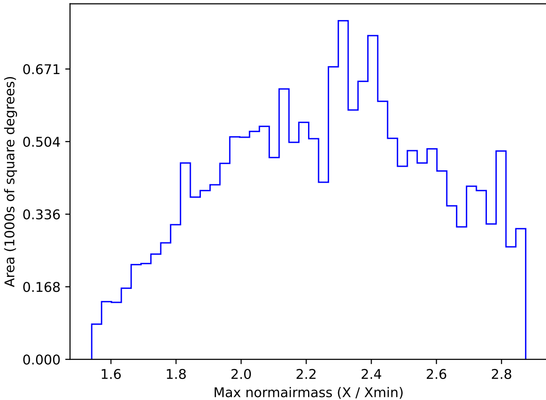
ddf_loaded_fl4_v3.4_10yrs WFD i band: Max normairmass
