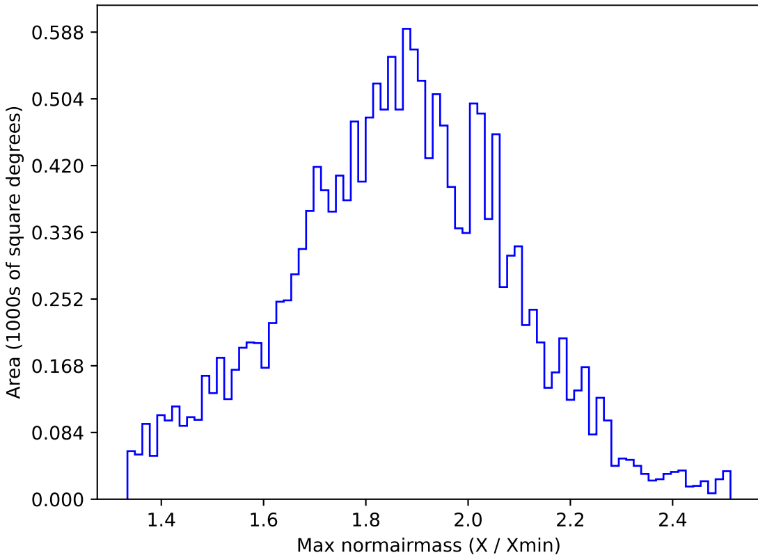
ddf_loaded_fl4_v3.4_10yrs WFD g band: Max normairmass
