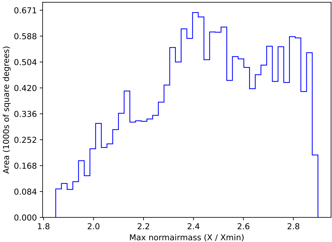
ddf_loaded_fl4_v3.4_10yrs WFD all bands: Max normairmass
