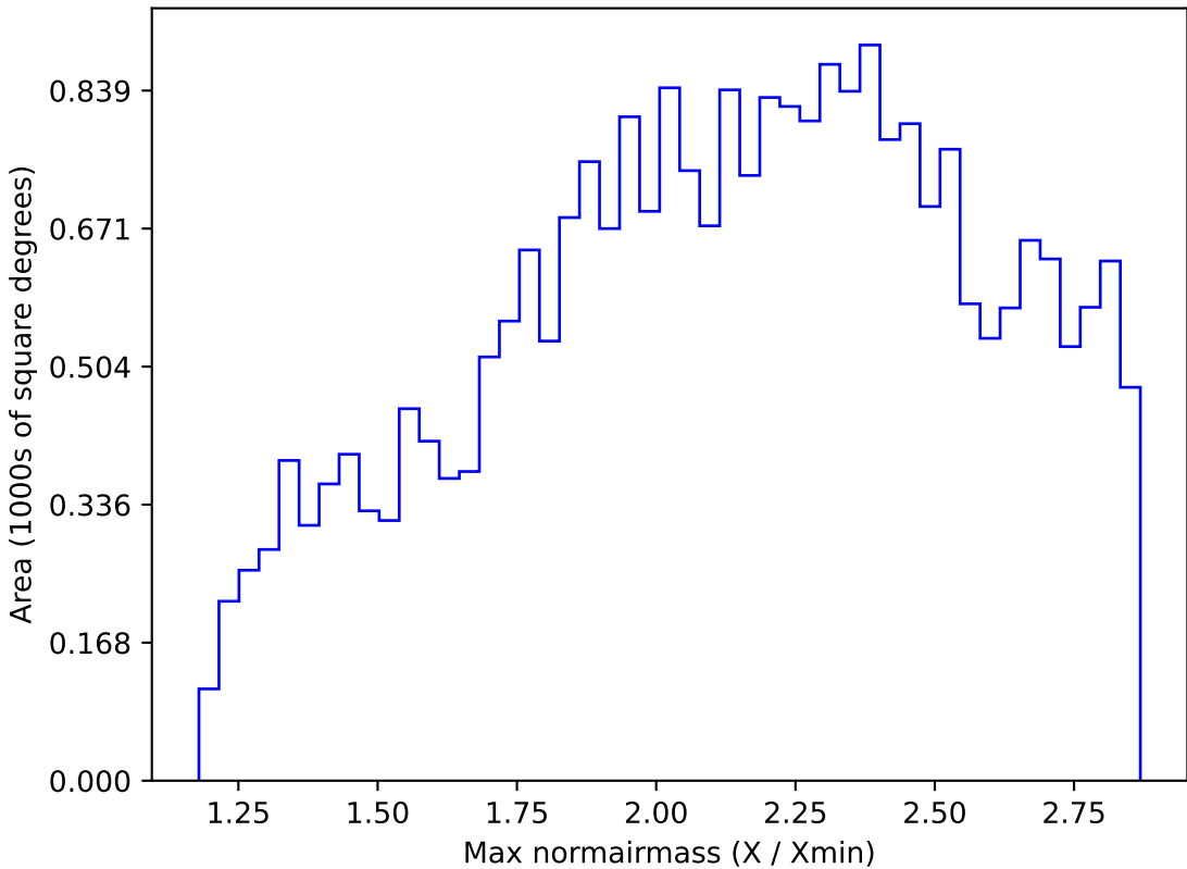
ddf_loaded_fl4_v3.4_10yrs All sky z band: Max normairmass
