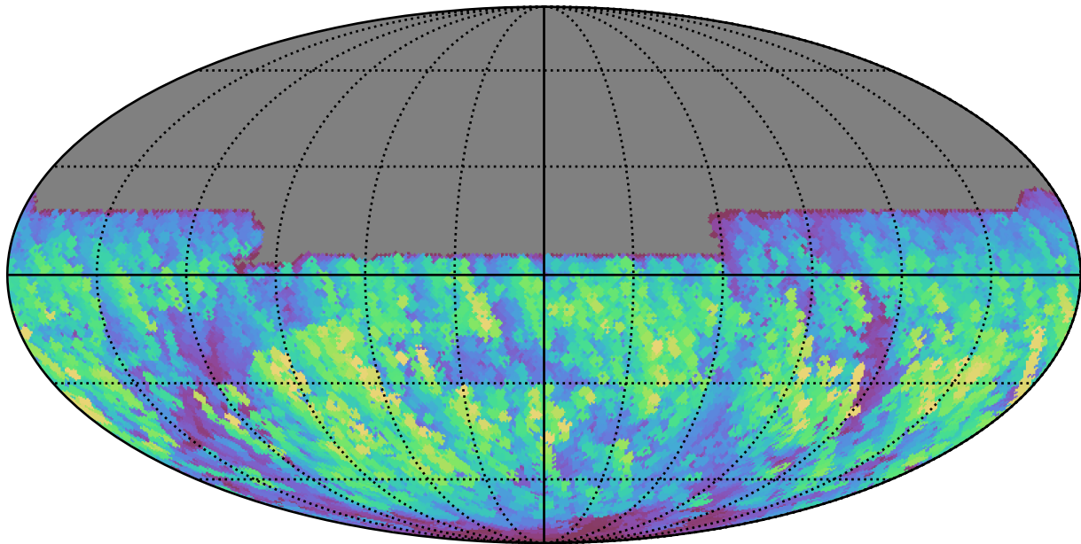
ddf_loaded_fl4_v3.4_10yrs All sky y band: Max normairmass
