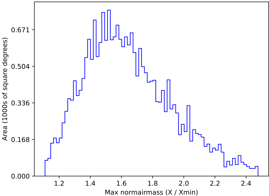
ddf_loaded_fl4_v3.4_10yrs All sky u band: Max normairmass
