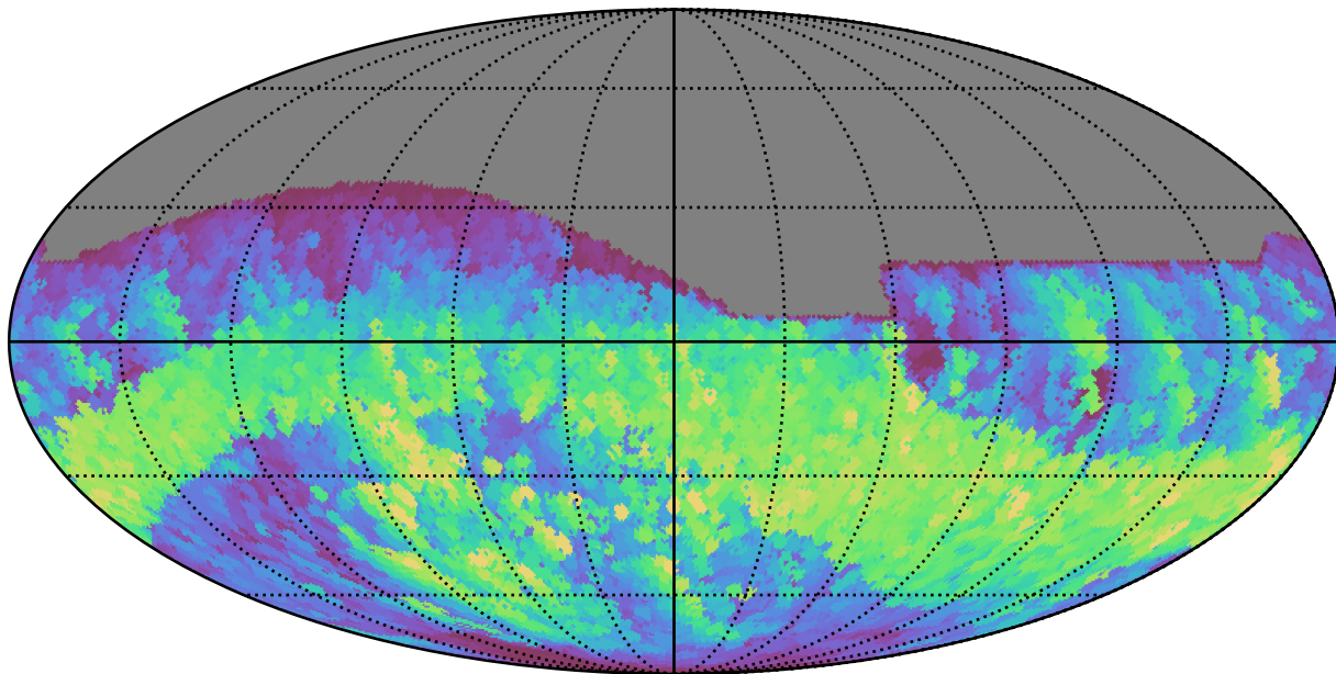
ddf_loaded_fl4_v3.4_10yrs All sky r band: Max normairmass
