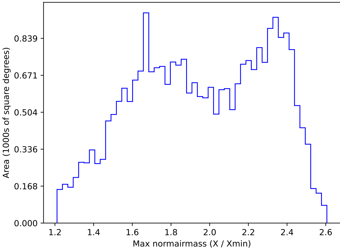
ddf_loaded_fl4_v3.4_10yrs All sky r band: Max normairmass
