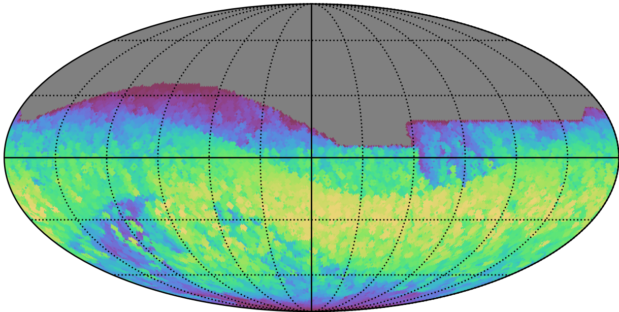
ddf_loaded_fl4_v3.4_10yrs All sky all bands: Max normairmass
