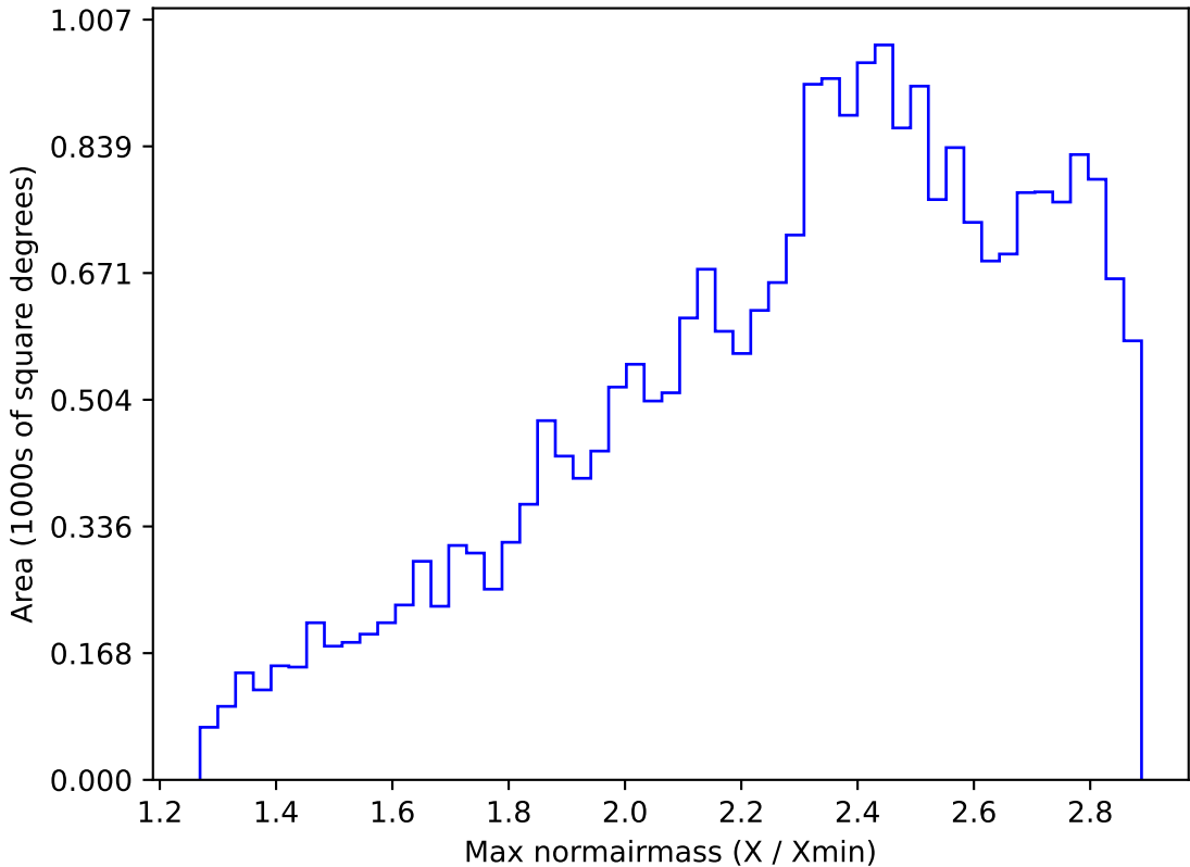
ddf_loaded_fl4_v3.4_10yrs All sky all bands: Max normairmass
