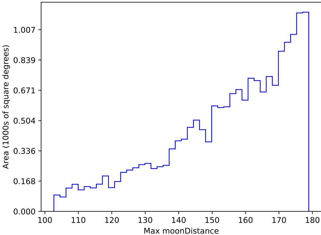
ddf_loaded_fl4_v3.4_10yrs WFD z band: Max moonDistance
